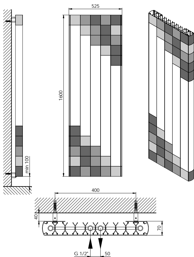
BITHERM Defile 525/1600
