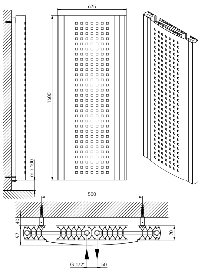
BITHERM Techno 675/1600
